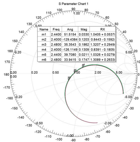
Figure 49. Chip antenna Smith chart after matching circuit usage
