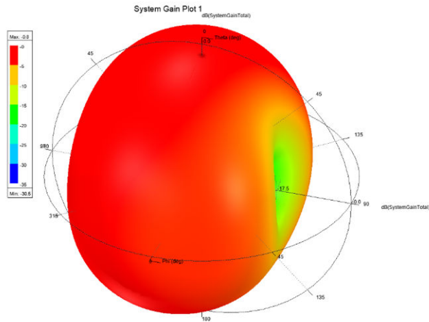
Figure 54. 3D gain radiation pattern of antenna 1 including axes
