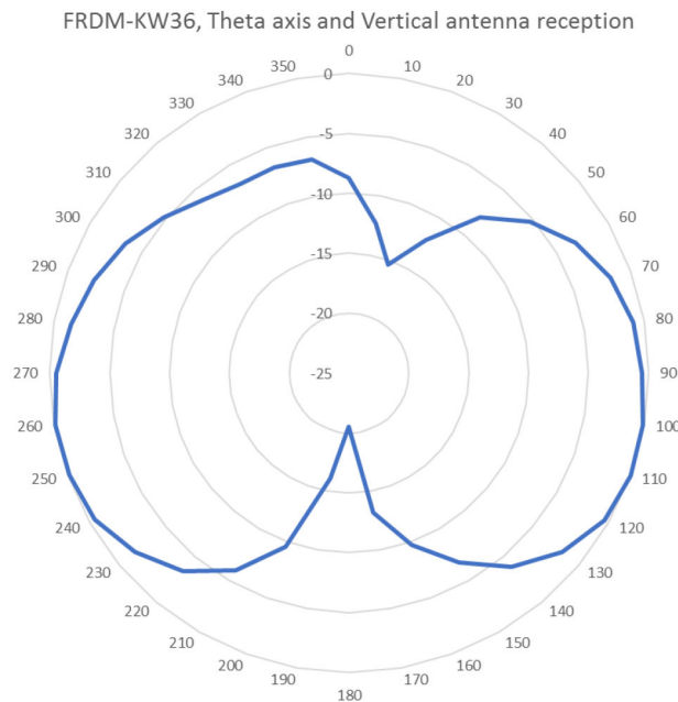
Figure 18. IFA antenna – gain and directivity diagram in Theta axis, maximum gain at 110° and 260°
