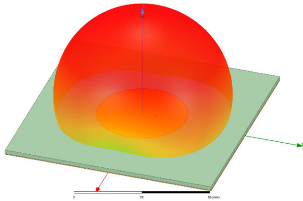
Figure 41. 3D gain radiation pattern of circular patch antenna with PCB
