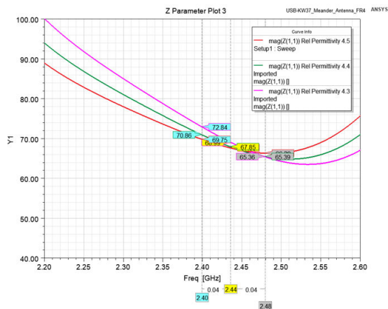
Figure 28. USB dongle – meandered PIFA antenna input impedance
