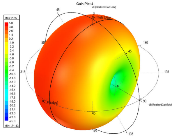
Figure 23. 3D gain radiation pattern of USB dongle board including angle axis
