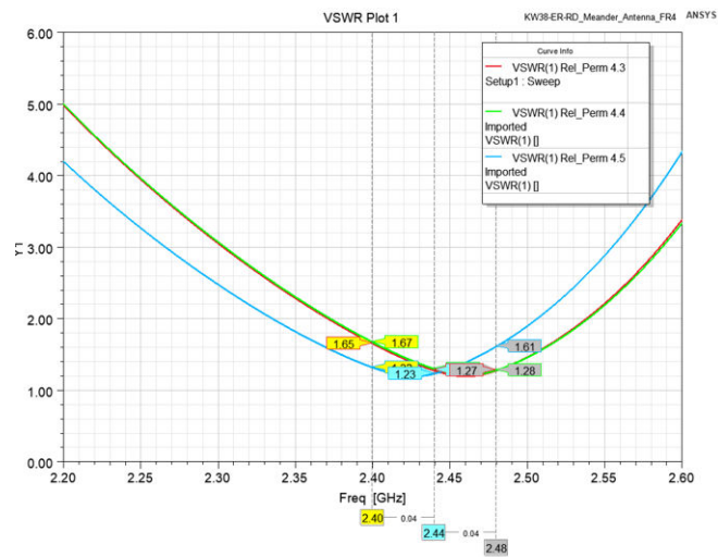
Figure 32. Extended-range board – meander antenna VSWR
