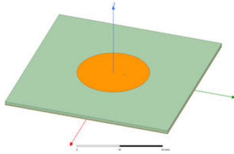
Figure 33. Circular patch antenna model with PCB example
