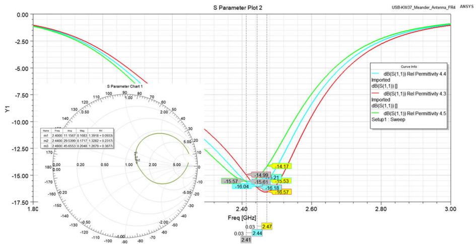
Figure 27. USB dongle meander antenna – reflection coefficient S11 with Smith chart, S11 varies with relative permittivity
