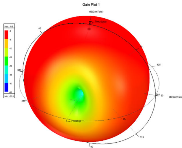
Figure 55. 3D gain radiation pattern of antenna 2 including axes
