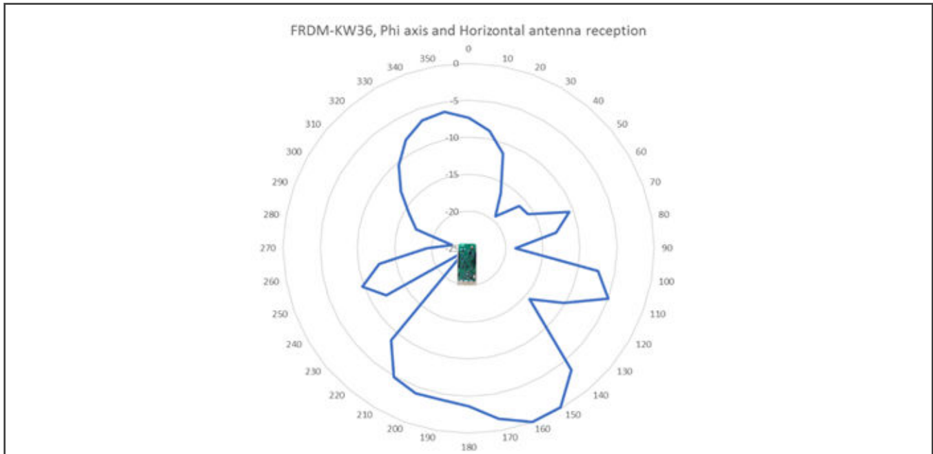
Figure 13. IFA antenna – gain and directivity diagram in Phi axis, maximum gain at 155°
