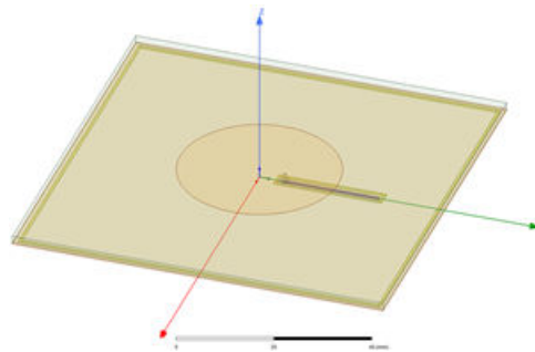
Figure 34. Circular patch antenna model with coaxial probe and feeding line on the bottom
