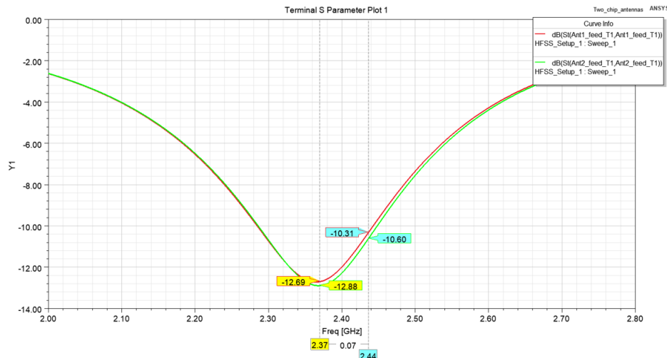
Figure 45. Chip antenna reflection coefficient – before matching
