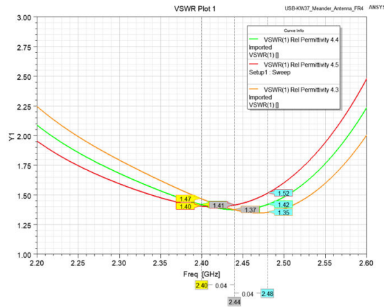
Figure 29. USB dongle – meandered PIFA antenna VSWR
