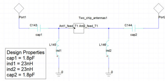
Figure 46. Example of the chip antenna matching circuit
