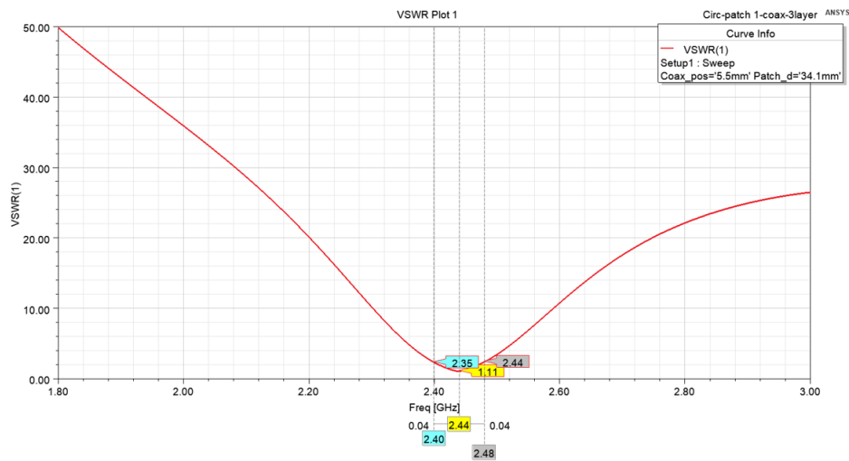
Figure 39. Circular patch antenna – VSWR
