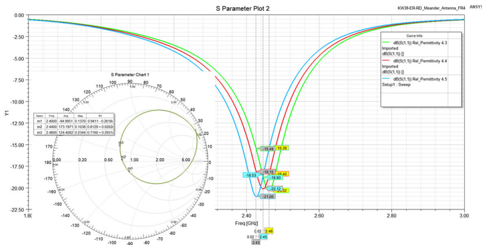
Figure 30. Extended-range board – meandered PIFA antenna reflection coefficient S11 with Smith chart, S11 varies with relative permittivity
