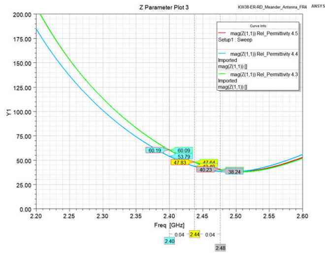
Figure 31. Extended-range board – meander antenna impedance
