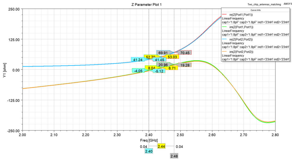
Figure 50. Johanson 2450AT42A100 chip antenna – impedance after matching
