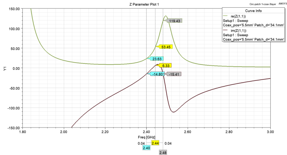
Figure 38. Circular patch antenna – impedance
