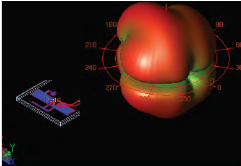
Figure 71. Total gain for all directions
