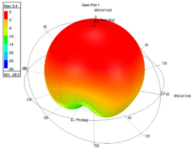
Figure 40. 3D gain radiation pattern of circular patch antenna
