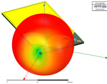
Figure 53. 3D radiation pattern of Johanson chip antenna 2 with PCB
