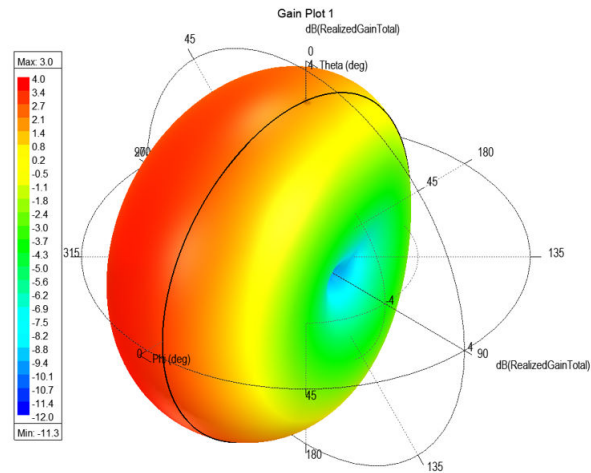
Figure 24. 3D gain radiation pattern of extended-range board including angle axis
