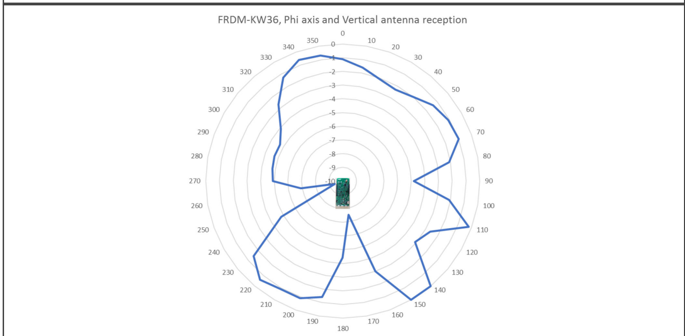
Figure 14. IFA antenna – gain and directivity diagram in Phi axis, maximal gain at 145°
